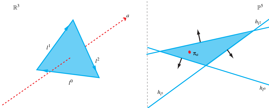
Figure 2: Left: a triangle in 3D space. l^0, l^1, l^2 are the lines spanning the triangle's edges. a is a line stabbing the triangle. Right: h_{l^0}, h_{l^1} and h_{l^2} are the Plücker hyperplanes mapped from l^0, l^1 and l^2 . \pi_a is the Plücker point mapped from the stabbing line a . \pi_a has a consistent orientation in respect to l^0, l^1 and l^2 . From a geometrical point of view, \pi_a lies at the intersection of the halfspaces induced by h_{l^0}, h_{l^1} and h_{l^2} . Thus, these 3 hyperplanes provide an analytical representation of all the lines stabbing the triangle.
