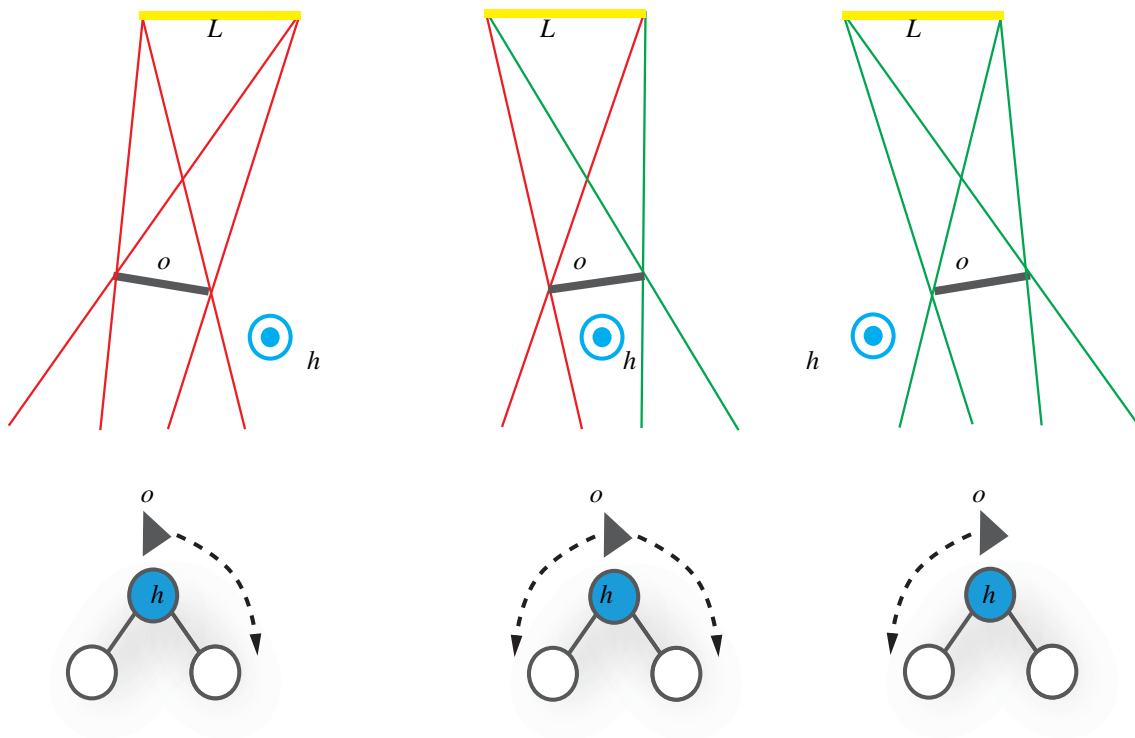
Figure 5: A 2D illustration of an insertion. An occluder o intersects a subset of all the lines originating from the light L . This subset may have a negative (first case), a mixed (second case), or a positive (third case) orientation in respect to a hyperplane h from an inner node. As a consequence the occluder o is inserted into the right, or both, or left subtree of the node. When a leaf is reached, the occluder is stored into the leaf except if it is an invisible class.
