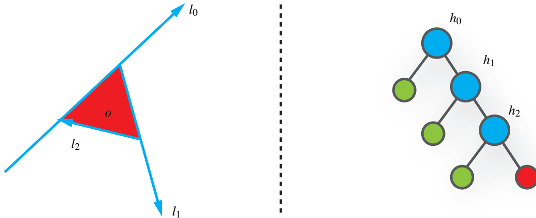
Figure 4: Let l_0, l_1, l_2 be the lines defined by the edges of an occluder o , and h_0, h_1, h_2 their dual hyperplanes in Plücker space. We can build a BSP tree whose leaves are the four equivalence classes generated by the triangle: Three visible classes (left leaves) and one invisible class (right leaf). We note bsp(o) such a representation.
