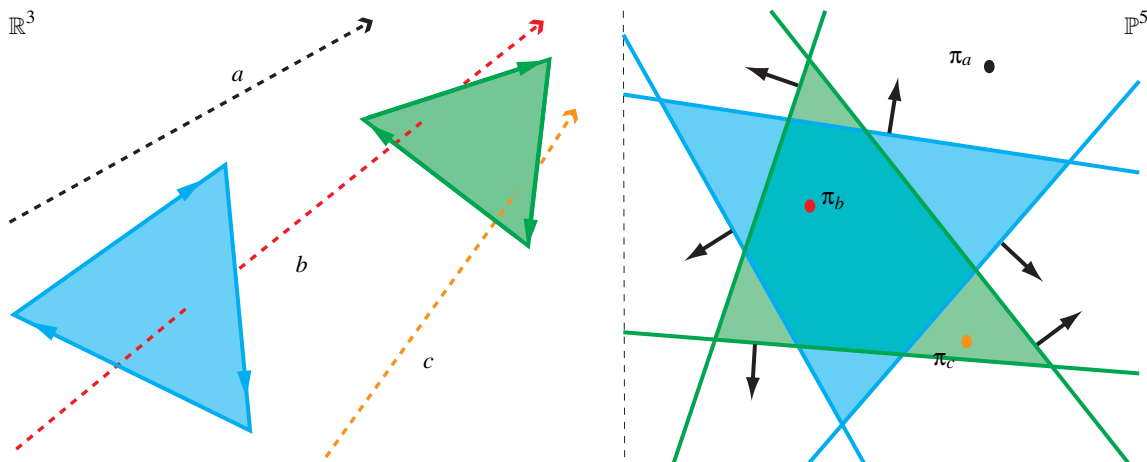
Figure 3: Left: 2 triangles and 3 lines a, b, c in various configurations. Right: The arrangement of hyperplanes (illustrated by 6 2D lines) mapped from the 6 triangles edges. They divide the Plücker space into cells. Filled cells are set of lines intersecting at least one triangle. \pi_a, \pi_b and \pi_c are the Plücker points mapped from a, b and c . They are located in the cells they belong to, according to the triangle(s) they stab. For example, \pi_b has a consistent orientation in respect to the 6 hyperplanes since b intersects the two triangles. Its relevant cell holds all the lines intersecting the two triangles.
