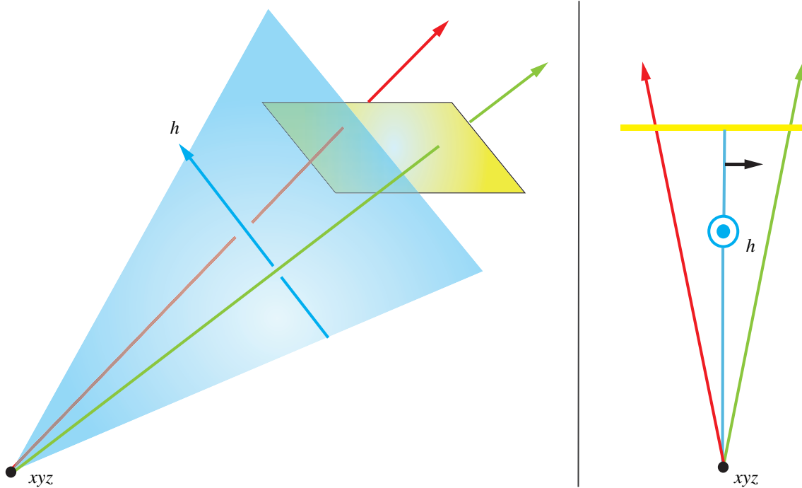
Figure 6: The point xyz and the line h define a plane that sets apart the lines having a positive or negative orientation in respect to h
