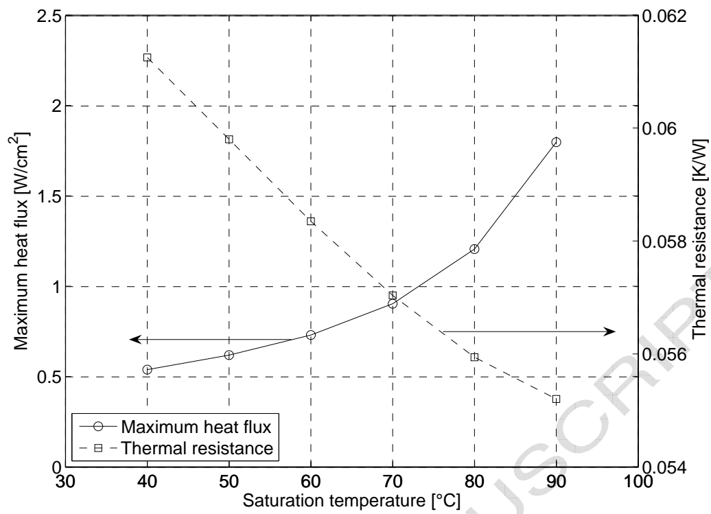
Figure 9. Effect of the saturation temperature on the maximum heat transfer capability and the overall thermal resistance.
