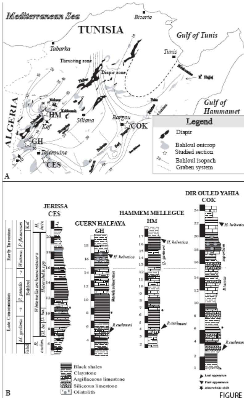
Figure 1 Location of the studied sections, (A) Bahloul isopach map and C/T palaeogeography in Central Tunisia (B) Stratigraphy and biostratigraphy of Jerissa (CES), Guern Halfaya (GH), Hammem Mellegue (HM) and Bargou (COK) sections.
