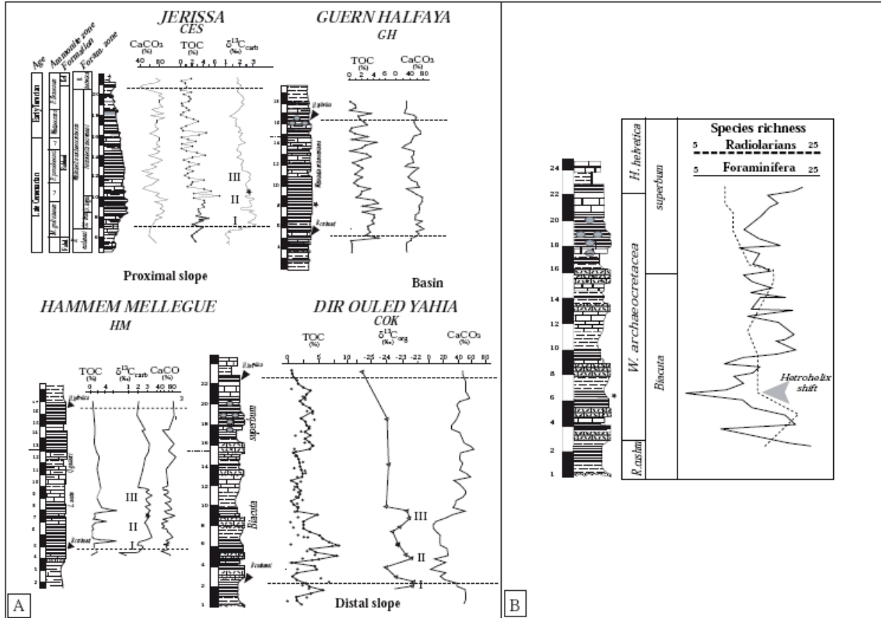
Figure 5 A. Geochemical (% \text{CaCO}_3 ; %TOC and % \delta^{13}\text{C} ) and biostratigraphic (foraminifera, radiolarians and ammonites) data of the four studied sections (modified from Souza and Tribouillard, 2007). I, II and III indicate the three worldwide isotopic spikes of the C/T boundary. Black stars indicate the Heterohelix shift (within each section). B. Distribution and correlation of foraminiferal and radiolarian profiles in the same graphic at Bargou section
