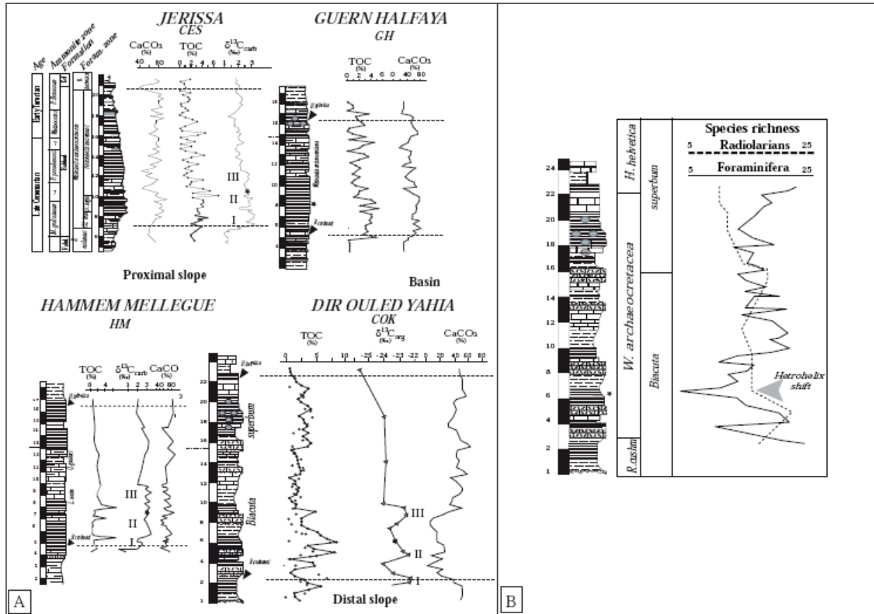
Figure 5 A. Geochemical (%CaCO 3 ; %TOC and %δ 13 C) and biostratigraphic (foraminifera, radiolarians and ammonites) data of the four studied sections (modified from Soua and Tribouvillard, 2007). I, II and III indicate the three worldwide isotopic spikes of the C/T boundary. Black stars indicate the Heterohelix shift (within each section). B. Distribution and correlation of foraminiferal and radiolarian profiles in the same graphic at Bargou section
