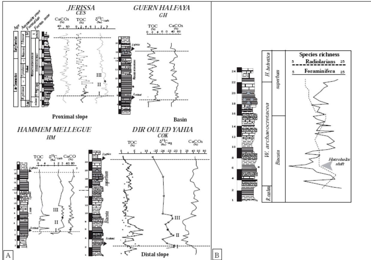
Figure 5 A. Geochemical (% \text{CaCO}_3 ; %TOC and % \delta^{13}\text{C} ) and biostratigraphic (foraminifera, radiolarians and ammonites) data of the four studied sections (modified from Soua and Tribouvillard, 2007). I, II and III indicate the three worldwide isotopic spikes of the C/T boundary. Black stars indicate the Heterohelix shift (within each section). B. Distribution and correlation of foraminiferal and radiolarian profiles in the same graphic at Bargou section
