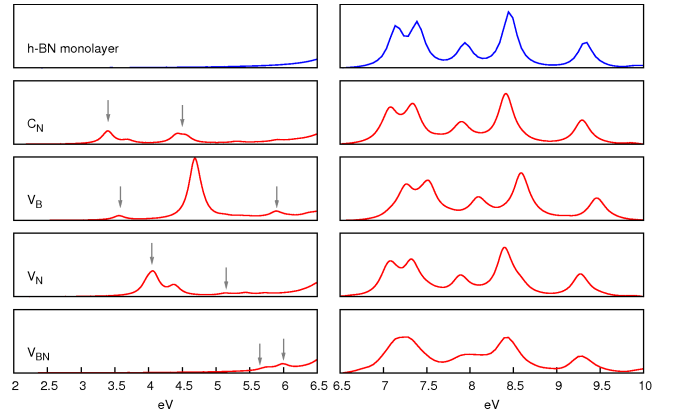
FIG. 3. Independent-particle absorption spectra (arbitrary units) based on the G_0W_0 quasi-particle band structure. In the left panel, the absorption cross section is increased by a factor 15 with respect to the right panel in order to make the defect-related peaks visible. .
