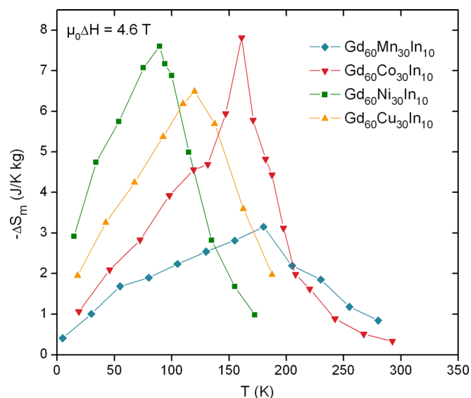
FIG. 5. (Color online) Temperature dependence of the isothermal magnetic entropy change \Delta S_m with a magnetic field change of 4.6 T, of melt-spun ribbons Gd 60 M 30 In 10 , M = Mn , Co, Ni, and Cu.
