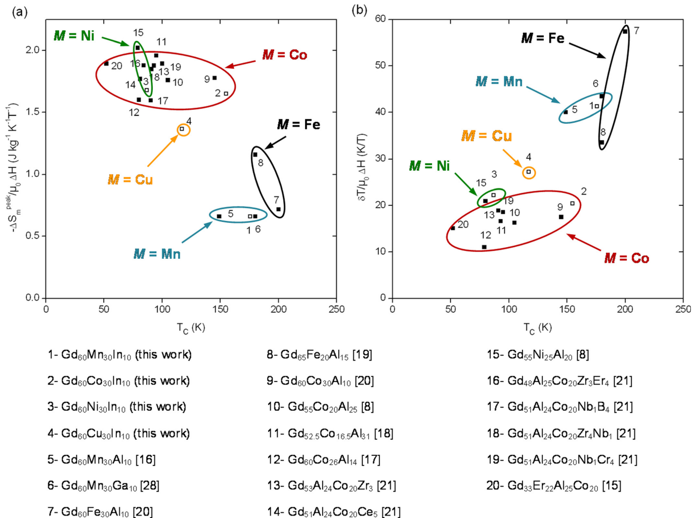
FIG. 6. (Color online) Maximal value of isothermal magnetic entropy change divided by the magnetic field change -\Delta S_m^{\text{peak}}/\mu_0 \Delta H (a) and temperature width at half maximum value of the magnetic entropy change divided by the magnetic field variation \delta T/\mu_0 \Delta H (b) vs T_C of melt-spun ribbons \text{Gd}_{60}\text{M}_{30}\text{In}_{10} , M = \text{Mn, Co, Ni, and Cu} (empty squares) and Gd-based metallic glasses from the literature (full squares).
