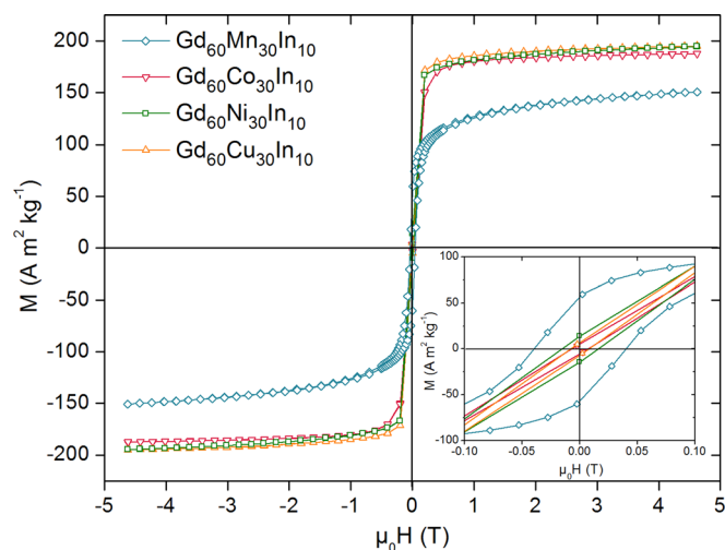
FIG. 4. (Color online) Field dependence between -4.6 and 4.6 T and at 5 K, of the magnetization M of melt-spun ribbons Gd 60 M 30 In 10 , M = Mn , Co, Ni, and Cu. The inset presents a zoom showing the coercive field and remanence of the samples.
