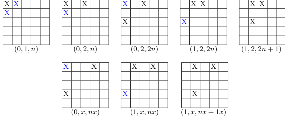
Fig. 9. From the configurations (0, 1, n) and (0, x, nx) with 2 \leq x \leq n - 1 .
