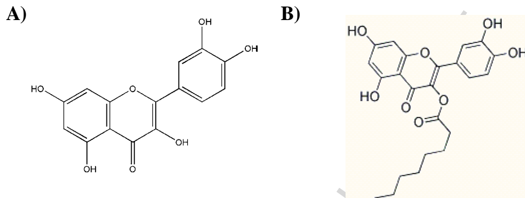
Figure 1: Chemical formula of A) QUER and B) QU-CAP.
