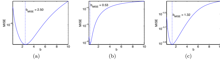
Fig. 4 MISE values as a function of b (from 1 replication) for (a): SeparatedBimodal. (b): Outlier. (c): AsymmetricClaw from n = 10^3 samples. The vertical dashed line represents the minimizer of the MISE.
