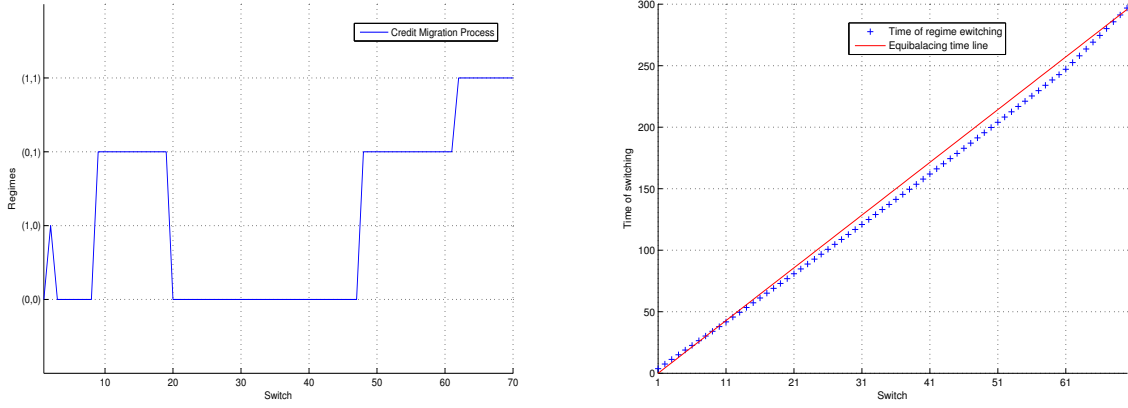
Figure 1: On left: Example of trajectory of the credit migration process X. On right: Example of instant of regime switching of the credit migration process X.
