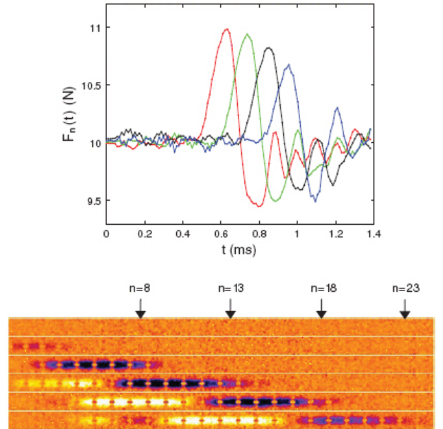
FIG. 4: (Color online) Top: Dynamical force F_n(t) vs time for grains n = 8, 13, 18, 23 (from the left to the right) in the linear regime. These curves are the result of the data analysis of photoelastic images by computing Eq. 4 for each grain. Before the pulse arises ( f_{1,max} = 1.3 \text{ N} for the first grain), each grain is submitted to the static force F_0 = 10 \text{ N} , then the pulse travels from one grain to another. The temporal width is quite constant for each grain but the maximal amplitude f_{n,max} decreases. Bottom: image sequence from which the curves have been determined. The grain used have been marked, we have divided the image by the first one of the movie, and used false colors.
