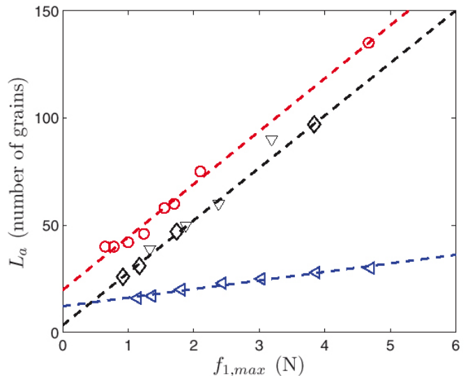
FIG. 12: (Color online) Distance of attenuation of the pulse given by Eq. (13) for different configurations: ( \diamond ) F_0 = 8\text{N} , F_{\perp} = 0.15\text{N/grain} , ( \nabla ) F_0 = 14\text{N} , F_{\perp} = 0.15\text{N/grain} , ( \circ ) F_0 = 26\text{N} , F_{\perp} = 0.22\text{N/grain} , ( \triangleleft ) F_0 = 26\text{N} , and F_{\perp} = 0.49\text{N/grain} . As predicted by Eq. (13), L_a increases linearly with f_{1,max} . The slope is 1/\alpha . It seems to not depend on F_0 but decreases when F_{\perp} increases.
