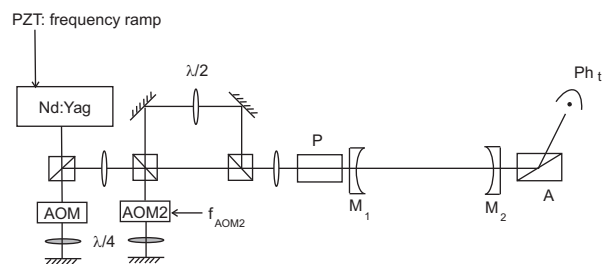
FIG. 7: Experimental setup for the cavity length measurement. Two laser beams frequency shifted one compared to the other by AOM2 are injected into the cavity. The frequency of the laser is frequency modulated with a voltage ramp applied on a piezo element mounted on the crystal resonator of the laser. Photodiode \text{Ph}_t allows to observe the typical Fabry-Perot peaks from which the FSR measurement is performed.
