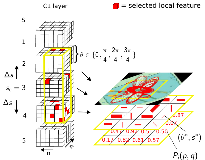
Fig. 3. HMAX-S multi-scale S2 prototype.
