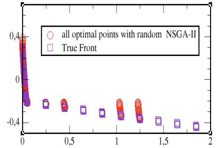
NSGA-II random
