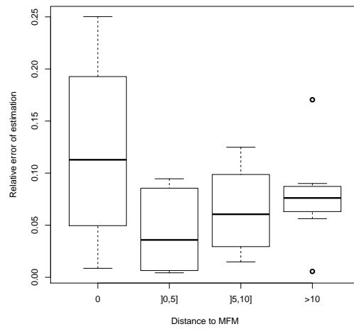
Fig. 5. Error of prediction of the number of proximity services jobs per inhabitant ( \frac{|Observed-Simulated|}{Observed} ). The large black line is the median while the box goes from the first quartile to the third quartile of the error distribution. The length of the horizontal line goes from the first decile to the nineteenth one. Circles represents the value above the nineteenth decile.
