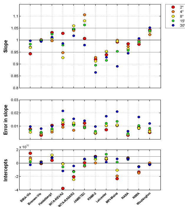
Fig. 11. Straight-line slopes and their standard errors and intercepts of \text{NO}_2 slant columns for each instrument participating in the semi-blind intercomparison at visible wavelengths against those of a reference data set. Colours refer to elevation angles shown in the top right legend. Note that the MPIC Mainz instrument used a non-standard wavelength range for spectral analysis because of the limited range of the instrument (Fig. 6 from Roscoe et al., 2010).
