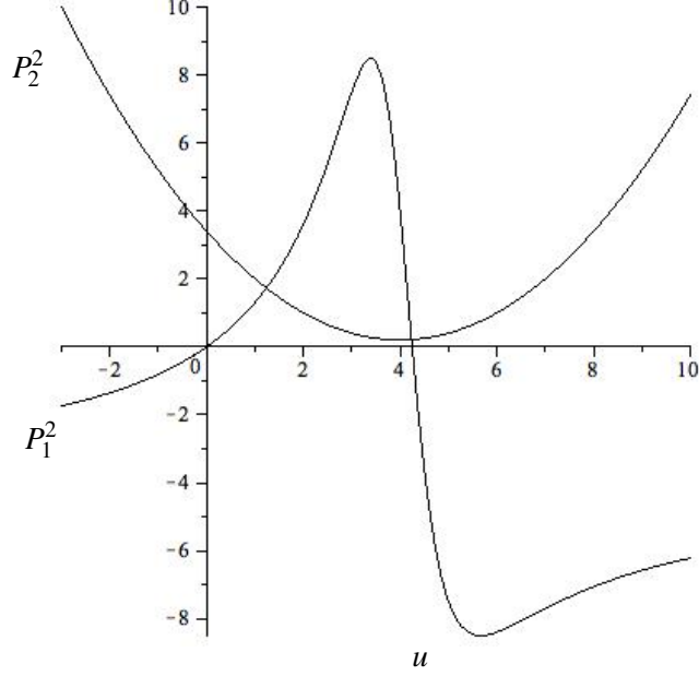
FIG. 8: Analytic Taub-NUT solution in terms of P_1 and P_2 for \mu = \beta = 1 .
