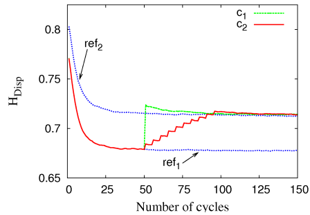
Fig. 7. Evolution of \mathcal{H}_{Disp} , and impact of peers arrival.
