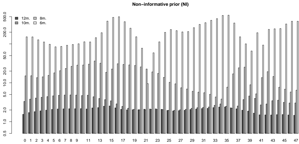
Figure 12: Using the non-informative prior: quality of the predictions (MAPE in %) averaged for each instant (all the 180 or so days within the prediction time-window are used for those averages), with an estimation period ranging from 12 to 6 months. The ordinate axis is in log-scale. Each shade of gray corresponds to a different scenario.
