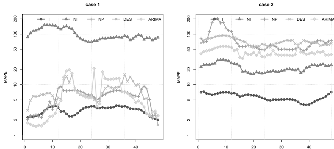
Figure 7: Quality of the predictions (MAPE in %) averaged for each instant, for both experiments: case 1 (left) and case 2 (right). The ordinate axis is in log-scale. Each shade of gray corresponds to one of the 5 methods tested.
