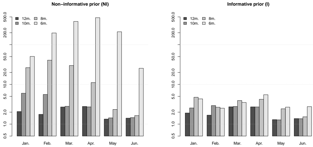
Figure 11: Quality of the predictions (MAPE in %) averaged for each month (all the instants of the 30 or so days within each month are used to compute these averages), with an estimation period ranging from 12 to 6 months using the non-informative prior (left) and using the informative prior (right). The ordinate axis is in log-scale. Each shade of gray corresponds to a different scenario.
