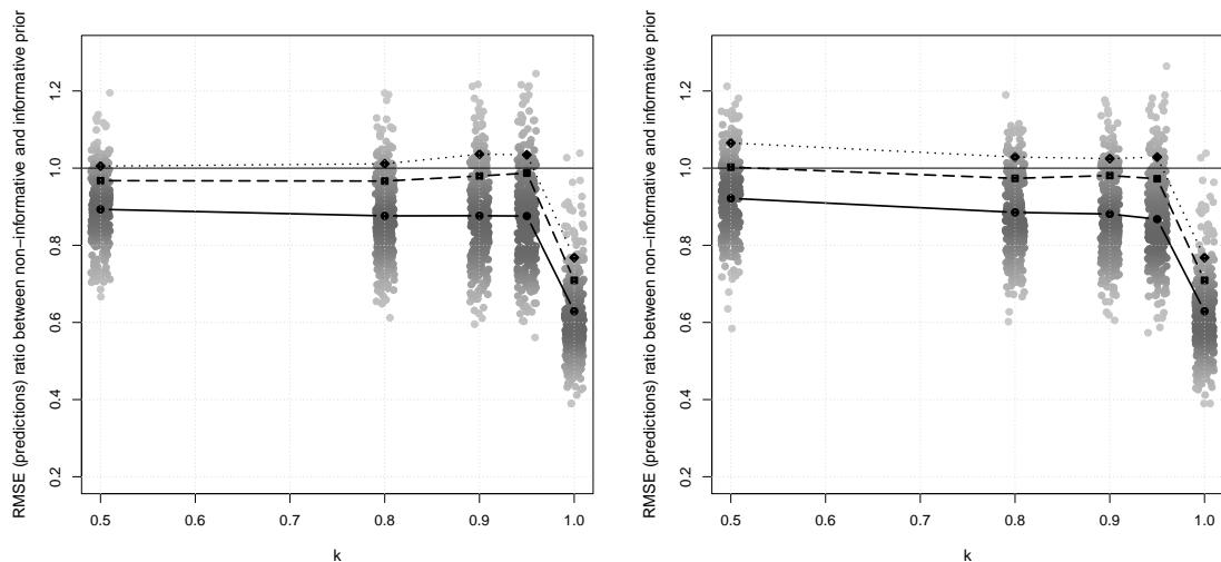
Figure 6: In grey: ratio between error predictions for the informative and the non-informative approach (abscissas have been jittered a bit to prevent overlapping, and different shades of grey are used to indicate the level of the estimated density). 300 replications for each value of k_\alpha = k_\gamma (left, where k_\beta = k_u = 1 ) and k_u (right, where k_\alpha = k_\beta = k_\gamma = 1 ) tested. In black: circles correspond to the averages, while squares and diamonds correspond to the 80% and 90% empirical quantiles of these ratios.
