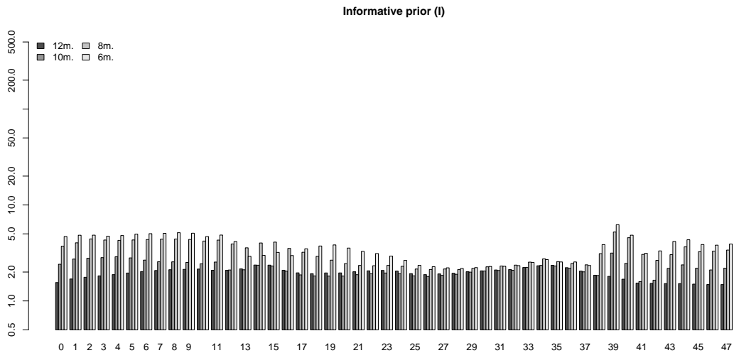
Figure 13: Using the informative prior: quality of the predictions (MAPE in %) averaged for each instant (all the 180 or so days within the prediction time-window are used for those averages), with an estimation period ranging from 12 to 6 months. The ordinate axis is in log-scale. Each shade of gray corresponds to a different scenario.
