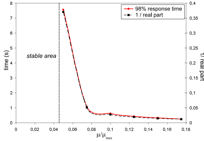
Figure 5: Evolution of the 98% response time with variations of the friction coefficient
