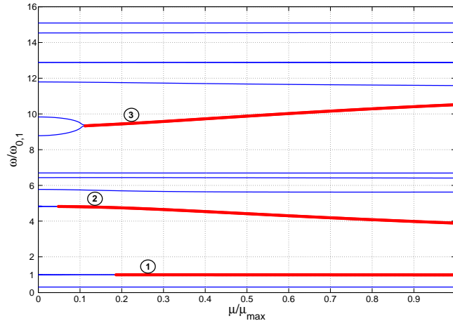
Figure 2: Angular pulsations versus friction coefficient
