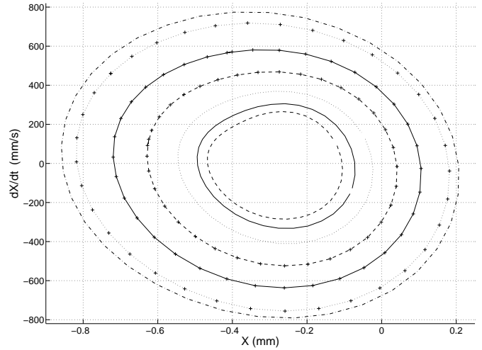
(b) End of the axle - vertical
