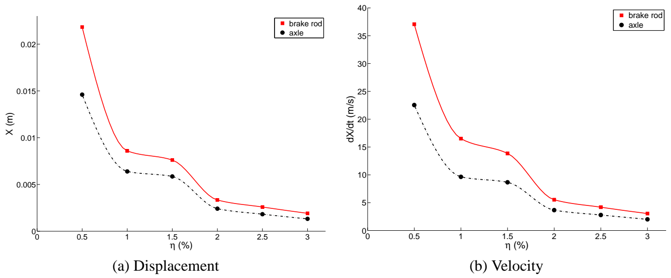
Figure 10: Vertical displacement of the axle - proportional damping
