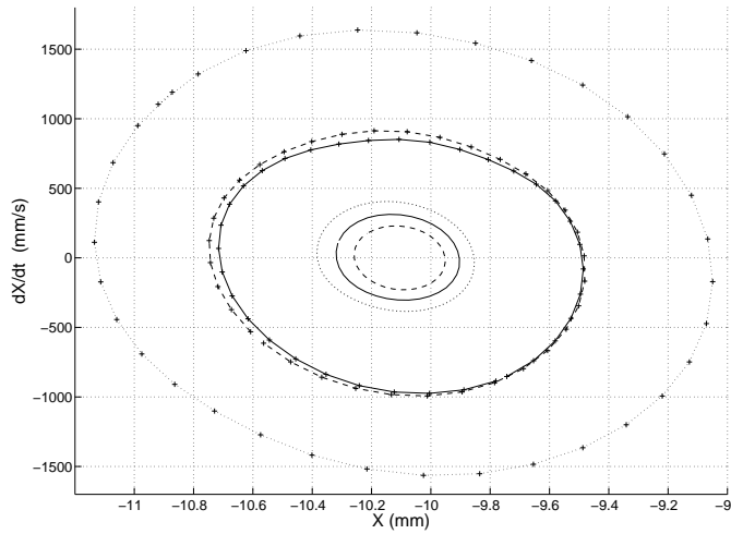
(a) End of the axle - horizontal
