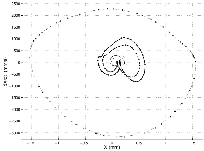
(c) Middle of the brake rod - horizontal
