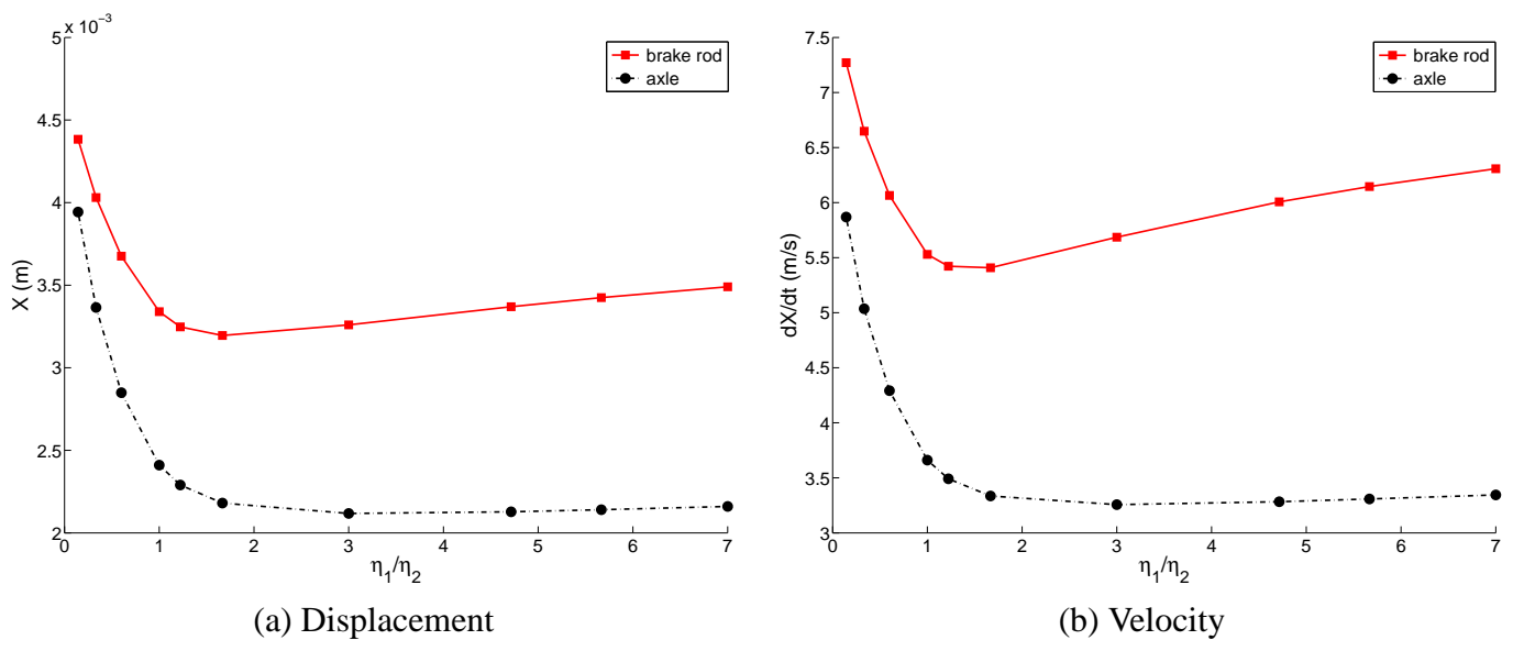
Figure 11: Vertical displacement of the axle - non-proportional damping
