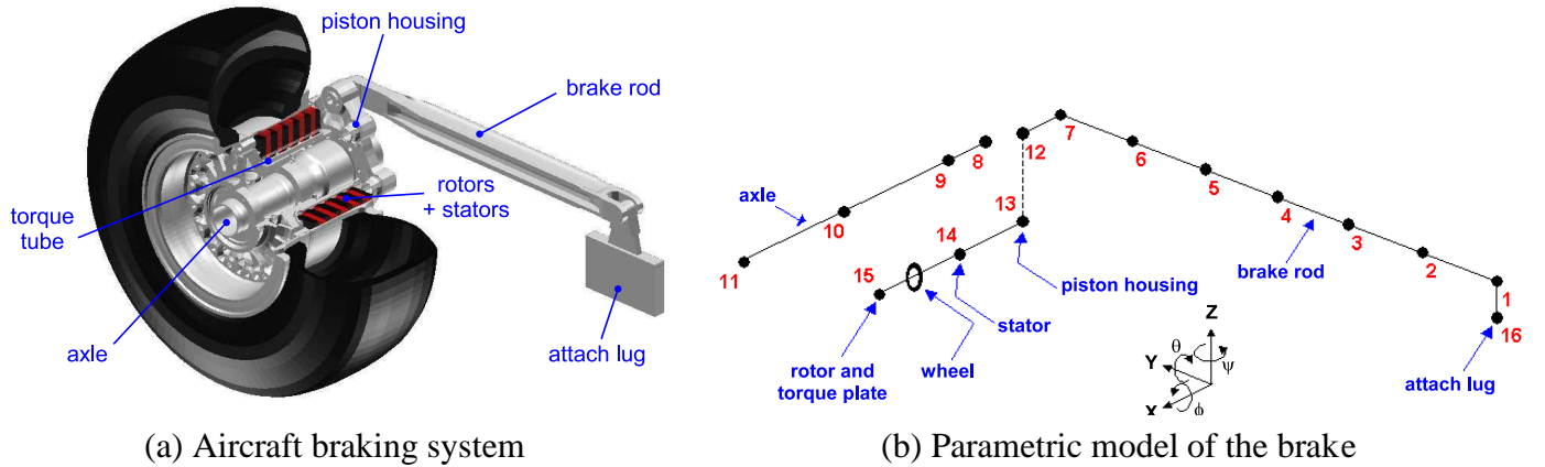
Figure 1: Aircraft braking system description
