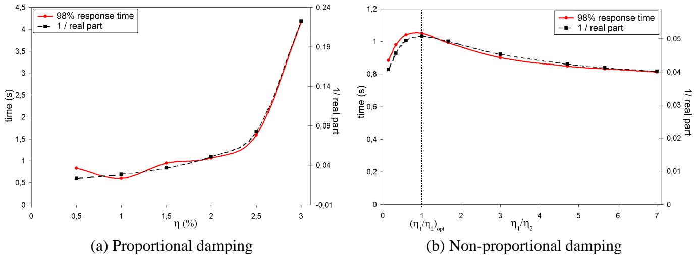
Figure 6: Evolution of the 98% response time with variations of damping
