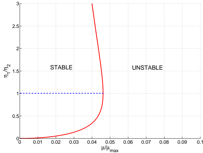
Figure 3: Stability (stable and unstable zones) versus \mu/\mu_{max} and \eta_1/\eta_2 for the second whirl instability
