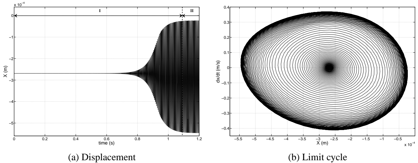
Figure 4: Vertical displacement of the axle ( \mu/\mu_{max} = 0.075 )
