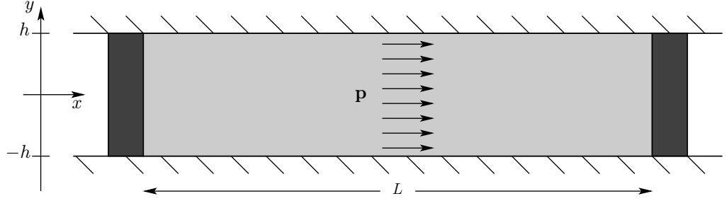
Figure 1. A thin film of active gel positioned between two pistons sets itself into motion.
