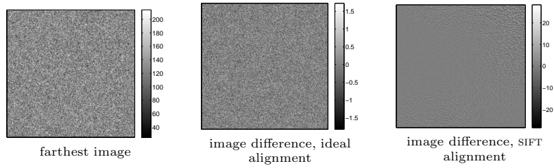
Figure 4: Synthetic example: 4\times PSF estimation for simulated data, residual image. From left to right: farthest image and residual images \mathcal{S}_s(\mathbf{H}_{\frac{\lambda}{s}} \tilde{\mathbf{v}}_1 * \mathbf{k}) - \tilde{\mathbf{v}}_2 with the estimated kernel from ideal and automatic alignment. The residual in the automatic alignment case is significantly larger than in the ideal alignment case. However, the difference in the PSFs seems to be negligible up to a subpixel translation as shown in Figure 3.
