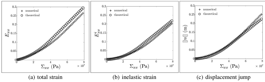
Fig. 12 Comparison between theoretical and numerical results - Mechanical response
