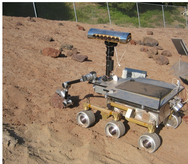
Figure 1. Rover Slope Slip Test
