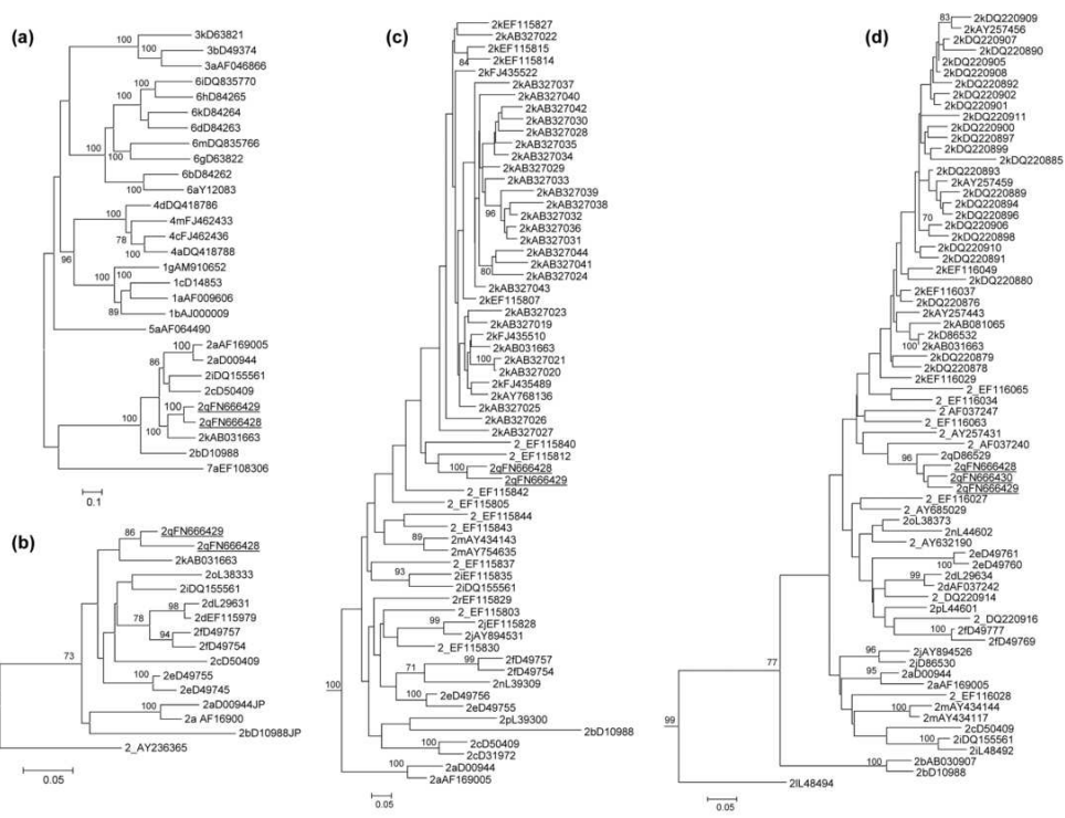
Figure 1. Maximum likelihood phylogenetic trees. (a) Unrooted phylogenetic tree of the coding region (positions 342 to 9336), nucleotide substitution model GTR + I + G (proportion of invariable sites: 0.301, gamma shape parameter: 0.841); (b) genotype 2 subtree of the Core region (positions 342 to 914), nucleotide substitution model GTR + I + G (proportion of invariable sites: 0.436, gamma shape parameter: 0.671); (c) genotype 2 subtree of the E1 region (positions 927 to 1262), nucleotide substitution model GTR + I + G (proportion of invariable sites: 0.436, gamma shape parameter: 0.671); (d) genotype 2 subtree of the NS5B region (positions 8283 to 8591), nucleotide substitution model GTR + I + G (proportion of invariable sites: 0.279, gamma shape parameter: 0.833). Positions are given according to the H77 reference sequence. Sequences are identified by genotype, subtype and GenBank accession number. Sequences that have not been assigned to any subtype are denoted as "2_". Sequences newly described in this study are underlined. Nodes supported by a bootstrap support value >70% are indicated. The scale bar represents number of substitutions per nucleotide position.
