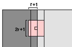
Figure 1: Toy example for computing \eta_{min} .
