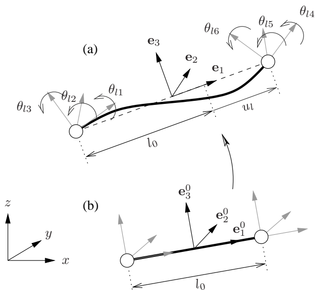
Figure 2: Illustration of the co-rotational approach: (a) current configuration, (b) initial configuration.
