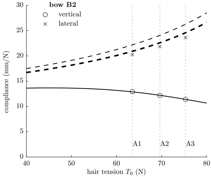
Figure 13: Evolution of vertical and lateral compliances at the tip ( \gamma = 1 ) with the hair tension on both bows, at a bow force of 1 N. The experimental values correspond to settings of hair-stick distance A1, A2, A3. Solid lines: simulated vertical compliance. Thin dashed lines: lateral compliance with a single equivalent hair representing the ribbon. Thick dashed lines: lateral compliance with n_h = 3 equivalent hairs.
