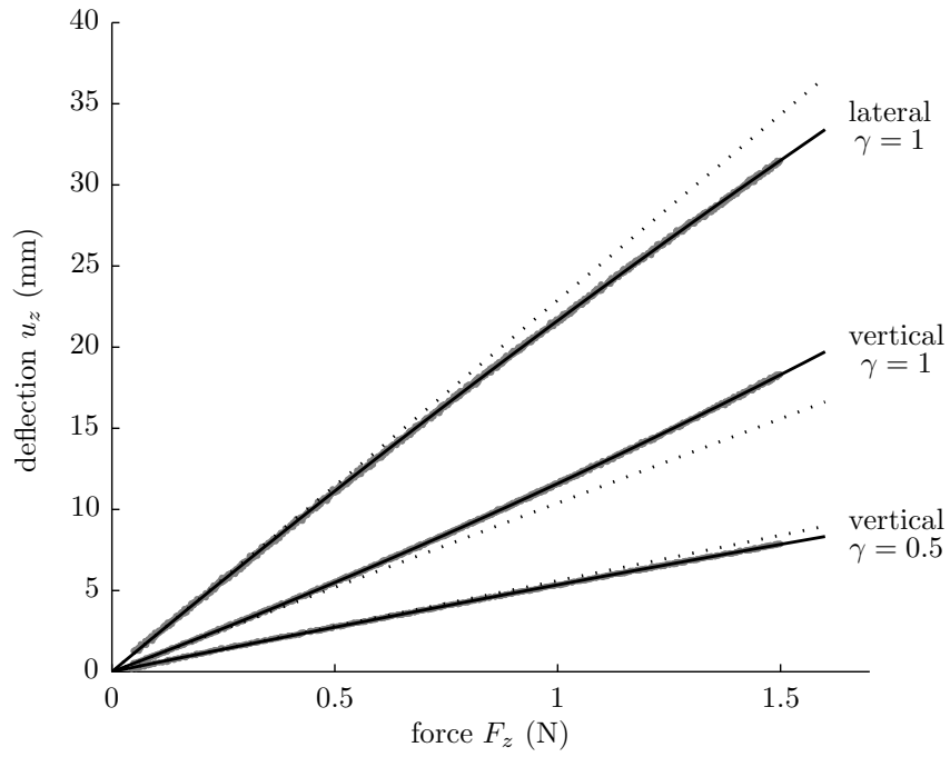
Figure 9: Measured force-deflection curves for three cases of loading on bow B2. Relative abscissa is denoted by \gamma ( \gamma = 0 at the frog, \gamma = 1 at the tip). Thick lines: experimental data. Thin lines: second order polynom. Dotted lines: linear relationship (tangent at F_z = 0 N).
