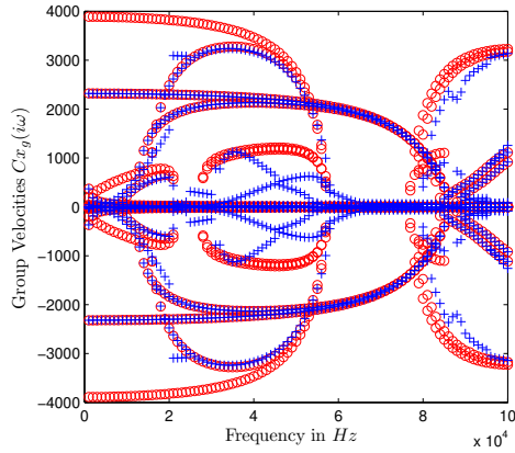
Figure 3. Group velocities along (Ox) direction; the red circles mark values obtained for Z = 0 and the blue crossed the optimal ones
