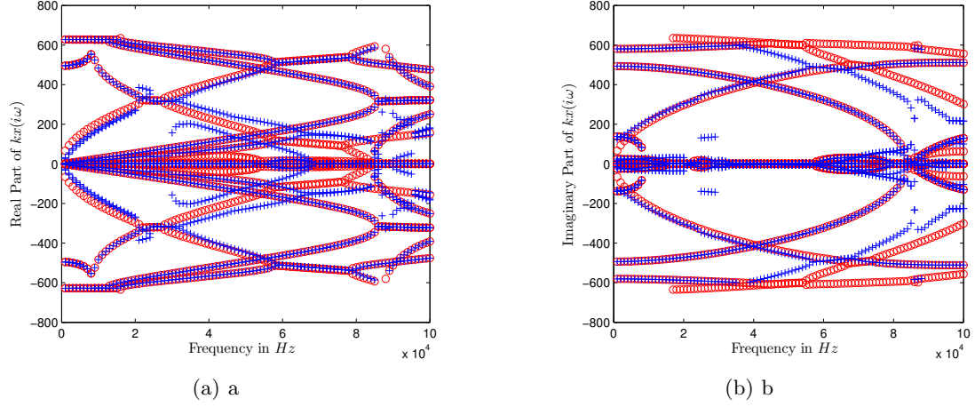
Figure 5. Real parts (a) and imaginary parts (b) of the wave number kx_n(i\omega) along (Ox) , the red circles mark values obtained for Z = 0 and the blue crossed the optimal ones
