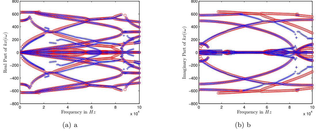
Figure 2. Real parts (a) and imaginary parts (b) of the wave number kx_n(i\omega) along (Ox) , the red circles mark values obtained for Z = 0 and the blue crossed the optimal ones
