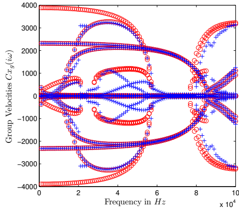
Figure 6. Group velocities along (Ox) direction; the red circles mark values obtained for Z = 0 and the blue crossed the optimal ones
