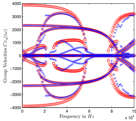
Figure 6. Group velocities along (Ox) direction; the red circles mark values obtained for Z = 0 and the blue crosses the optimal ones
