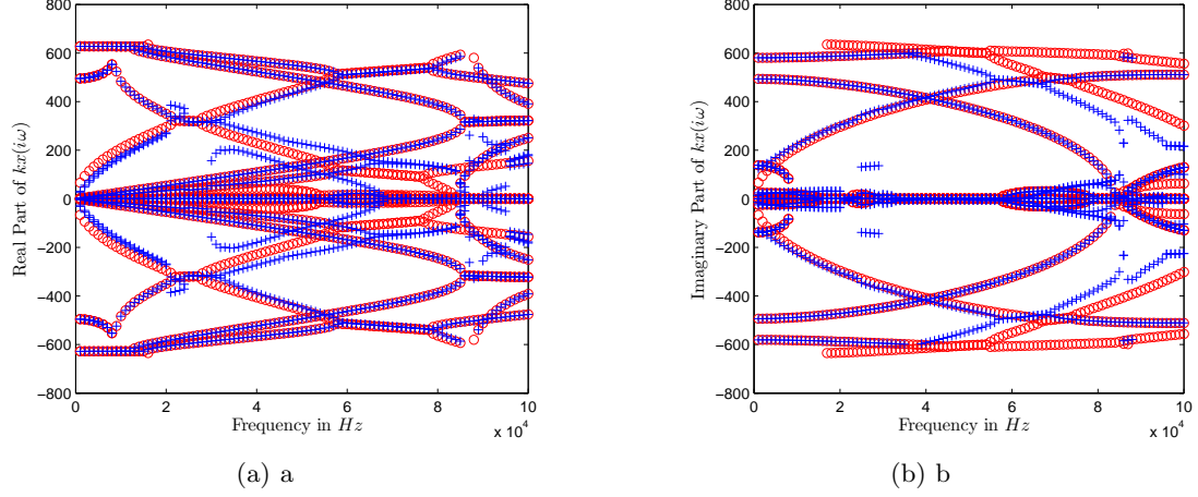
Figure 5. Real parts (a) and imaginary parts (b) of the wave number kx_n(i\omega) along (Ox) , the red circles mark values obtained for Z = 0 and the blue crossed the optimal ones
