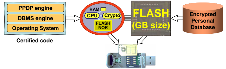
Fig. 2. SPT's internal architecture
