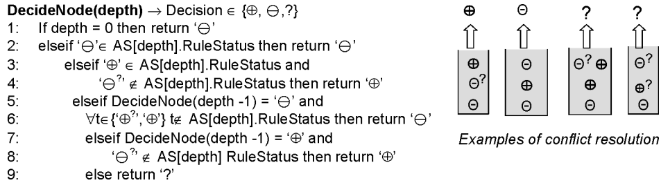
Fig. 4. Conflict-resolution algorithm.
