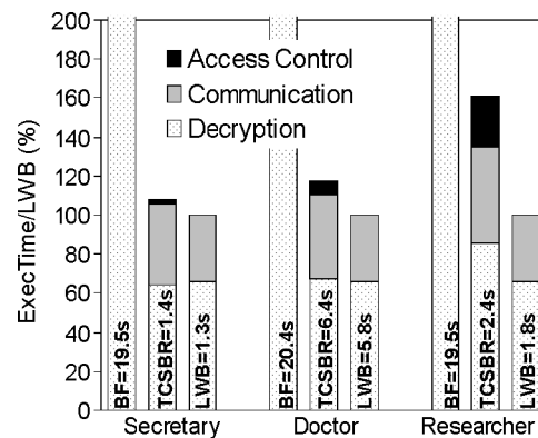
Fig. 12. Access-control overhead.
