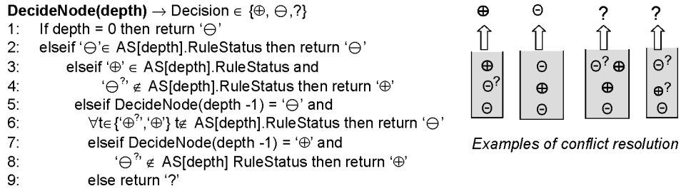
Fig. 4. Conflict-resolution algorithm.
