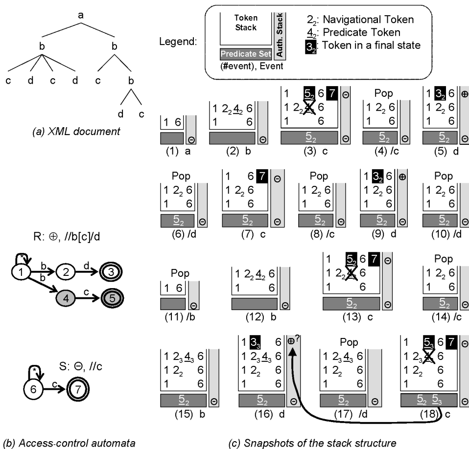
Fig. 3. Execution snapshot.
