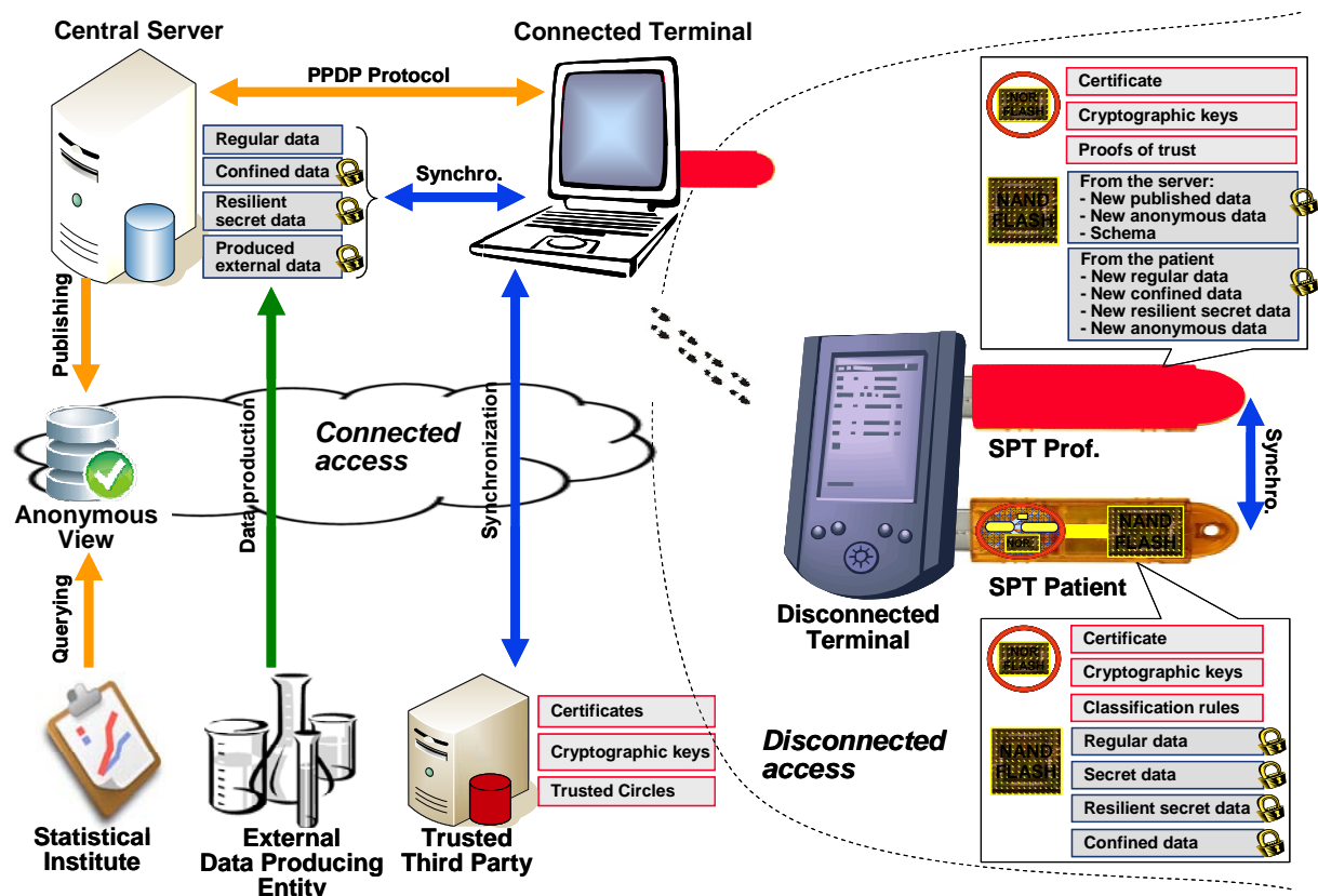
Figure 2. Functional architecture
