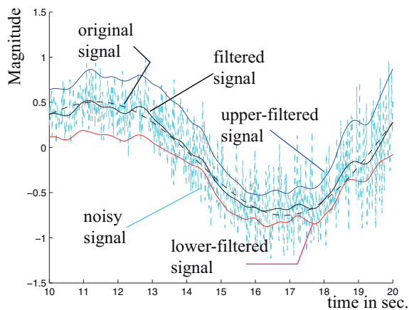
Figure 7: Imprecise signal filtered with the symmetric Choquet (Sipos) integral based approach.
