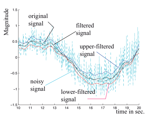
Figure 4: Precise signal filtered with the symmetric Choquet (Sipos) integral based approach.
