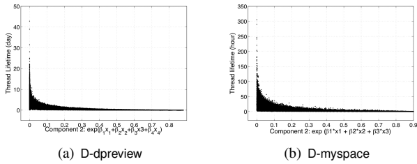
Figure 6: risk factor component ( x_1\beta_1 \dots x_k\beta_k ) vs. the lifetime of threads
