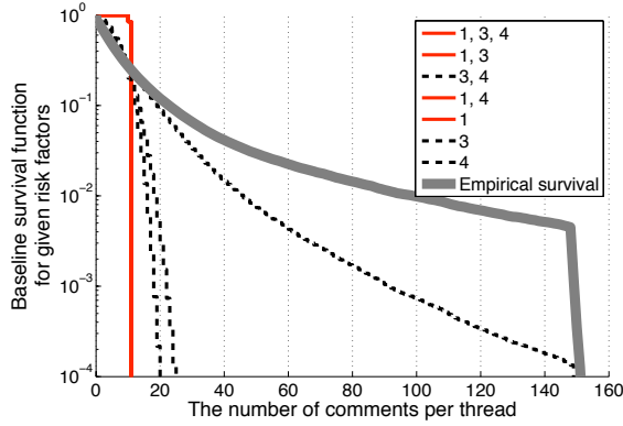
Figure 7: Predicting the number of comments of online discussion forum threads
