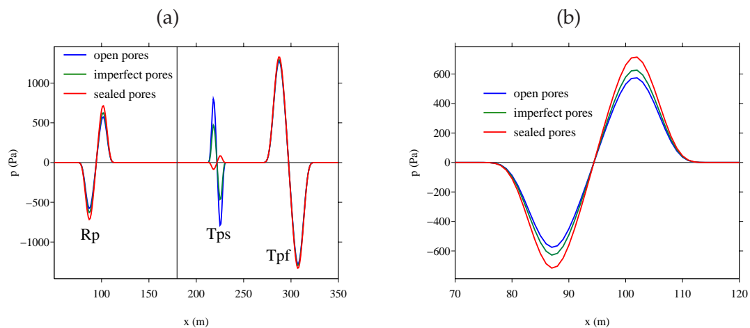
Figure 4: test 1. Slices of p at the final instant, for various interface conditions. (a): reflected acoustic wave R_p , transmitted fast compressional wave T_{pff} , transmitted slow compressional wave T_{ps} . (b): zoom around the wave reflected in the fluid domain ( R_p ).
