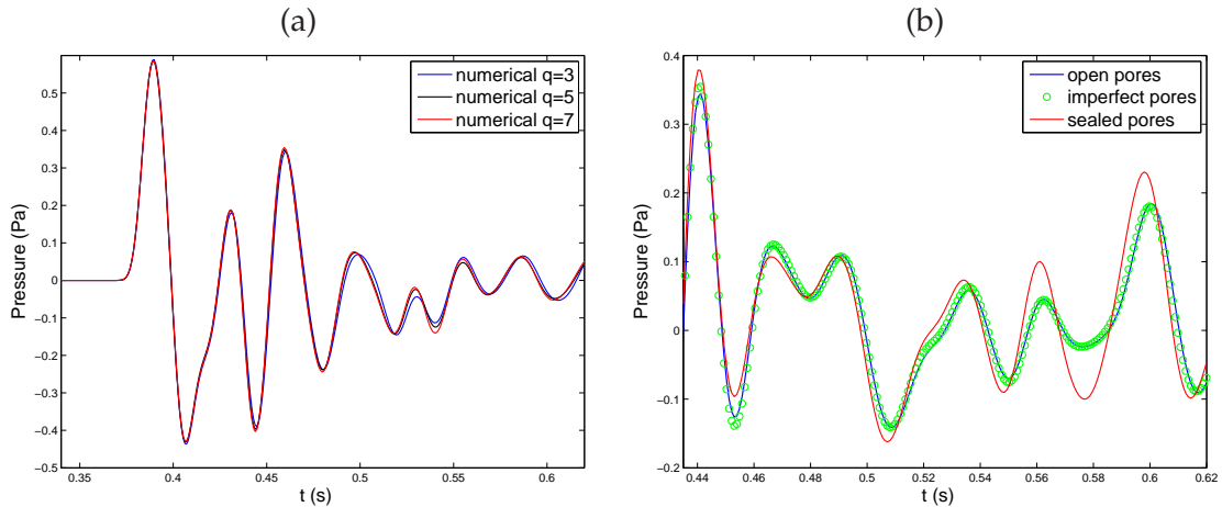
Figure 11: test 3. (a): time history of p at the receiver R1 in \Omega_1 for different refinement factors; time history of p at the receiver R0 in \Omega_0 , for t > 0.435 s (b).
