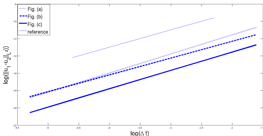
FIGURE 3. Strang method
