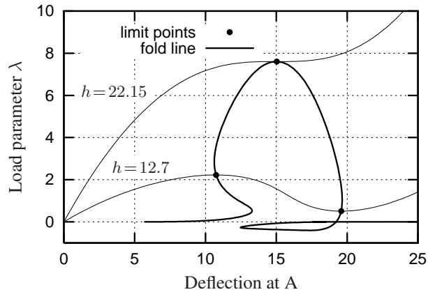
Figure 4. Fold line and equilibrium curves with associated limit points for different values of the thickness ( h = 12.7 and h = 22.15 )
