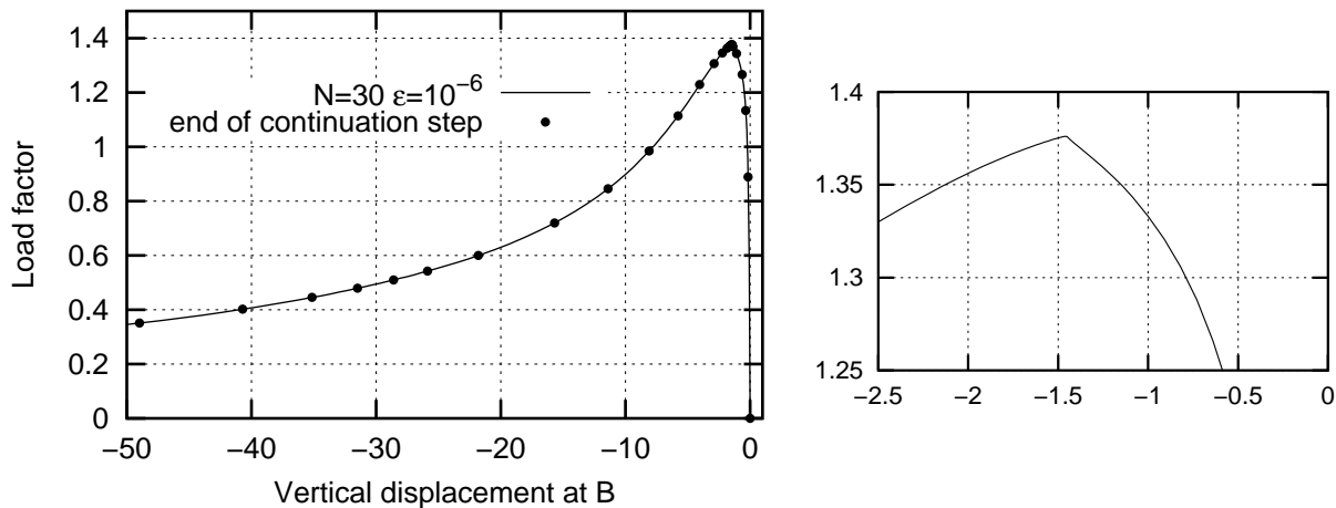
Figure 2: a) Load-displacement curve for the C-profile with an initial shape imperfection (global flexural mode) such that w_B = -0.1 . b) Magnification of the area near the limit point
