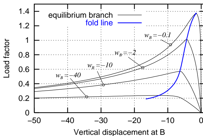
Figure 4: Fold line and equilibrium curves for different values of the imperfection amplitude.
