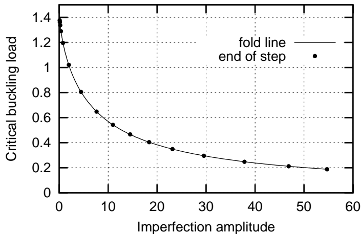
Figure 5: Reduction of the critical buckling load with respect to the amplitude of the shape imperfection.
