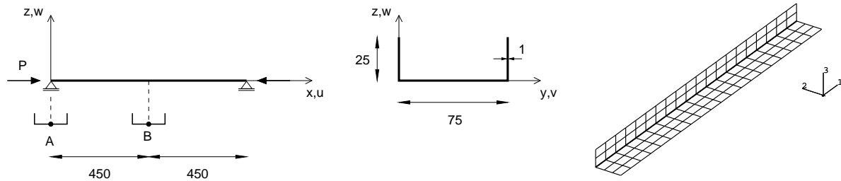
Figure 1: Geometrical properties and shell-element subdivision for one quarter of the C-profile. Material properties: E=2100000 , \nu=0.3 . Boundary conditions: u(0, 450, 0)=0 , v(0, 0, 0)=v(l, 0, 0)=0 , w(0, y, 0)=w(l, y, 0)=0
