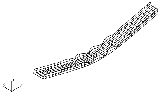
Figure 3: Deformed configuration of the complete C-profile along the post-buckling path.
