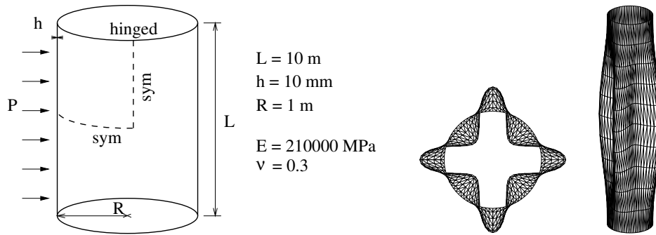
Figure 8: (a) Problem definition (b) First buckling eigenmode of the perfect cylinder (cross section and perspective)
