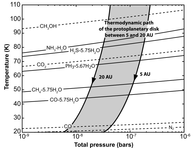
FIG. 2.— Equilibrium curves of hydrate (NH 3 -H 2 O), clathrates (X-5.75H 2 O or X-5.67H 2 O) (solid lines), pure condensates (dotted lines) and the ensemble of thermodynamic paths (grey area) ranging between 5 and 20 AU in the pressure-temperature space of the disk, assuming full efficiency of clathration. Species remain in the gas phase above the equilibrium curves. Below, they are trapped as clathrates or simply condense.
