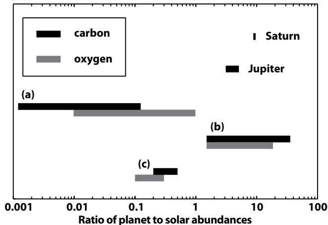
FIG. 1.— Carbon and oxygen abundances (relative to hydrogen) in HD 189733b compared with solar values. Elemental abundances derive from the analysis by MS09 (bars a) of the planet spectra acquired with Spitzer broadband photometry during secondary eclipses, and from the interpretation by MS09 (bars b) and S09 (bars c) of the same spectra obtained during dayside observations by HST NICMOS spectrophotometry in the 1.5–2.5 \mu\text{m} range. Carbon abundances measured in Jupiter and Saturn are shown for comparison (values taken from Mousis et al. 2009a). The oxygen abundance is still unconstrained in these two planets.
