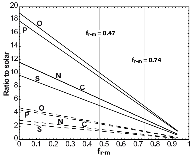
FIG. 3.— The volatile enrichments in the envelope of HD189733b as a function of the fraction of rocks and metals f_{r-m} in accreted planetesimals. Volatile enrichments have been calculated in the case of the presence of 20 M_{\oplus} (dashed lines) and 80 M_{\oplus} (solid lines) of heavy elements in the envelope, respectively. The two vertical lines enclose the range of plausible f_{r-m} values in planetesimals for which volatile enrichments are predicted in HD189733b (see text). N and C lines appear superimposed. If 80 M_{\oplus} of heavy elements is present in the envelope, our enrichment predictions are within the range of determinations of MS09 from HST NICMOS spectrophotometry, irrespective of the f_{r-m} value in the 0.47–0.74 range. If 20 M_{\oplus} of heavy elements is present in the envelope, the simultaneous fit of the O and C determinations by MS09 from HST NICMOS spectrophotometry leads to a unique common solution for f_{r-m} = 0.48 .
