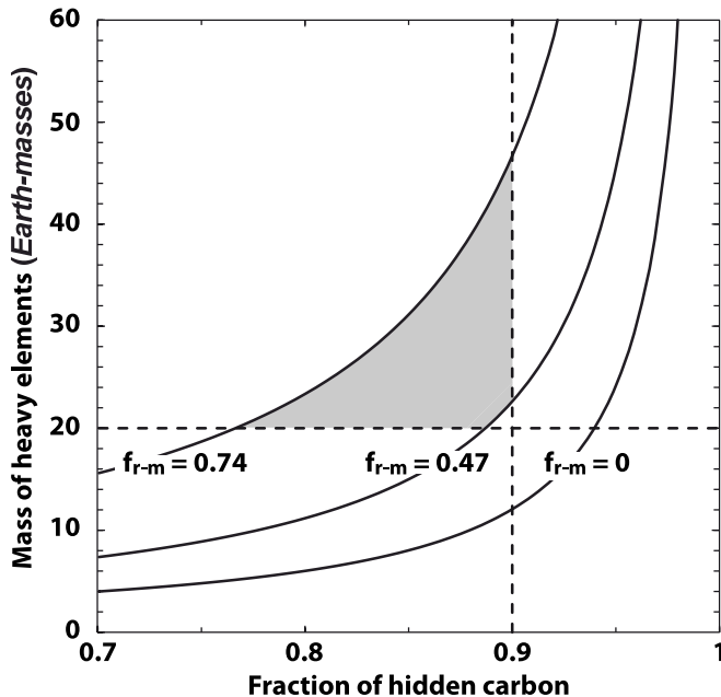
FIG. 4.— The mass of heavy elements in HD189733b as a function of the fraction of carbon hidden in the atmosphere (see text). The horizontal dashed line corresponds to the minimum mass of heavy elements predicted in HD189733b (Guillot 2008). The vertical dashed line corresponds to the upper value of the carbon fraction that can exist in the form of soots and organic molecules at sampled pressure levels. The three solid curves correspond to different fractions of rocks and metals f_{r-m} in planetesimals accreted by HD189733b during its formation (see text). The grey area represents the range of fractions of hidden carbon matching the global heavy element content predicted in HD189733b’s interior, which is enclosed by the two most plausible values of f_{r-m} , assuming a composition of planetesimals similar to those formed in the Solar nebula (see text).
