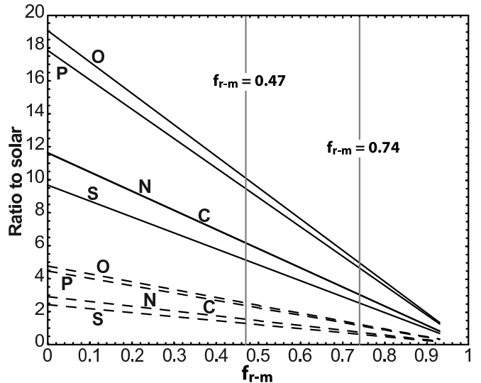
FIG. 3.— The volatile enrichments in the envelope of HD189733b as a function of the fraction of rocks and metals f_{r-m} in accreted planetesimals. Volatile enrichments have been calculated in the case of the presence of 20 M_{\oplus} (dashed lines) and 80 M_{\oplus} (solid lines) of heavy elements in the envelope, respectively. The two vertical lines enclose the range of plausible f_{r-m} values in planetesimals for which volatile enrichments are predicted in HD189733b (see text). N and C lines appear superimposed. If 80 M_{\oplus} of heavy elements is present in the envelope, our enrichment predictions are within the range of determinations of MS09 from HST NICMOS spectrophotometry, irrespective of the f_{r-m} value in the 0.47–0.74 range. If 20 M_{\oplus} of heavy elements is present in the envelope, the simultaneous fit of the O and C determinations by MS09 from HST NICMOS spectrophotometry leads to a unique common solution for f_{r-m} = 0.48 .
