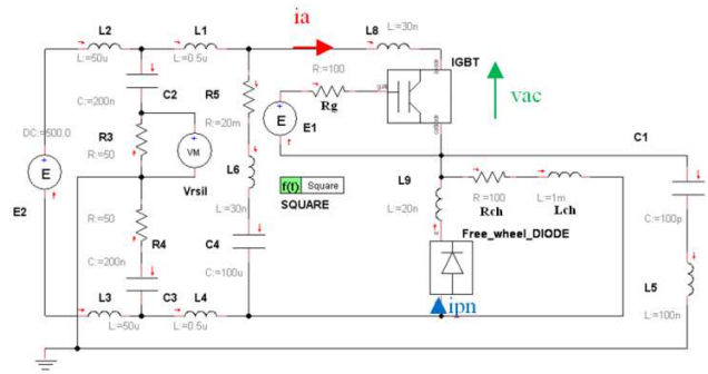
Figure 7: Switching circuit
