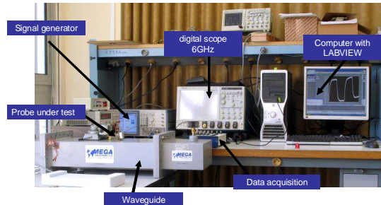
Figure 1: Test bench
