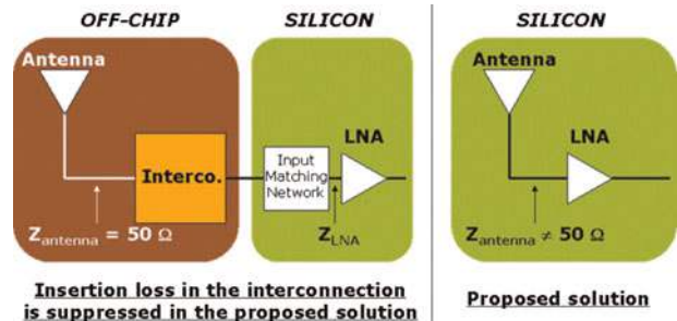
Fig. 4. Co-integration technique in an SoC approach.
