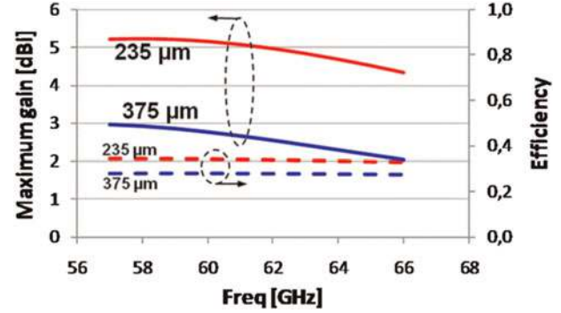
Fig. 10. Maximum gain and efficiency versus frequency.
