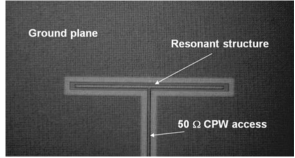
Fig. 13. Folded-slot antenna on a HR silicon substrate.
