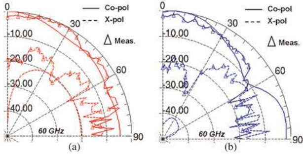
Fig. 12. Measured and simulated radiation pattern of the dipole antenna on 235 \mu\text{m} -height substrate: (a) E -plane and (b) H -plane.
