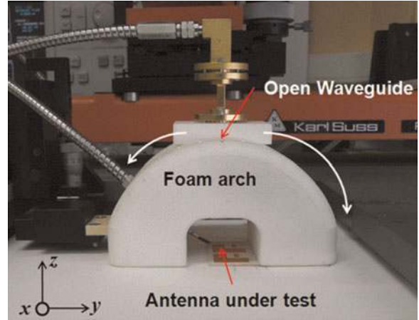
Fig. 3. Lab-STICC measurement setup for radiation pattern characterization.
