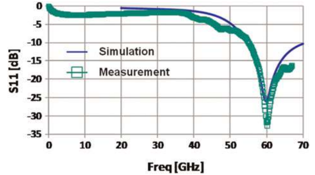
Fig. 14. Folded-slot antenna matching.
