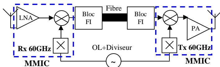
Figure 2. Architecture Tx/Rx
