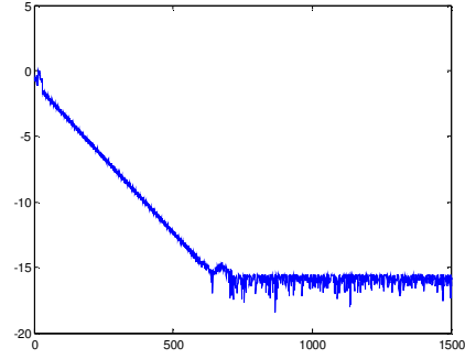
Figure 4. Quadratic synchronization error, asymptotic observer.
